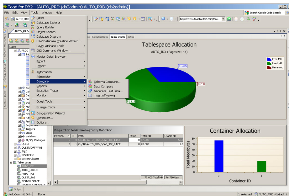
Simplified database administration and schema migration using Toad for IBM DB2
